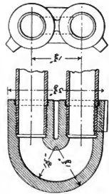
Figs. 500-506. Back End of Superheater Tubes.
